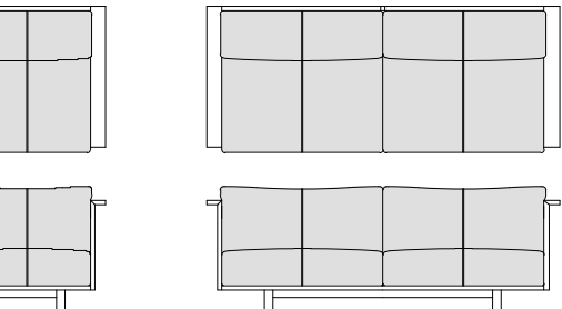
High Sofa 189 W189. D87.5. H75. SH38
