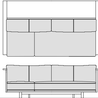
C Counter Sofa 221 W221. D126. H75. SH38
