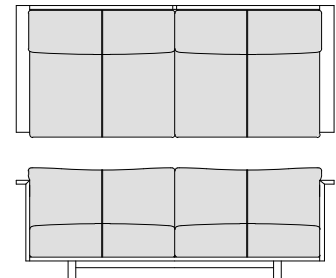
High Sofa 210 W210. D87.5. H75. SH38
