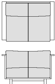
High Sofa 114 W114. D87.5. H75. SH38
