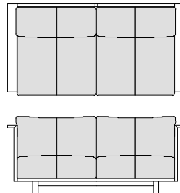
High Sofa 168 W168. D87.5. H75. SH38
