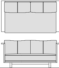
C High Sofa 158 W158. D87.5. H75. SH38
