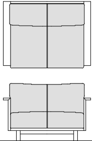
Sofa 114 W114. D87.5. H75. SH38
