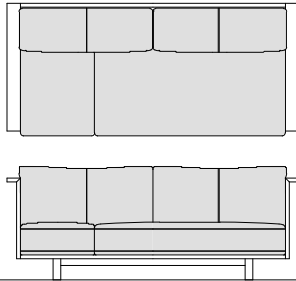
C High Sofa 193 W193. D87.5. H75. SH38
