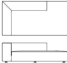
Couch 175 (Left) (Right) W175. D91. H56. SH35
